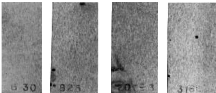
All four of these alloys were immersed in 4% NaCl + 0.1% Fe 2 (SO 4 ) 3 + 0.01M HCl at 122 deg. F (50°C) for 48 hours. HASTELLOY G-30 alloy was the only one not to pit.
